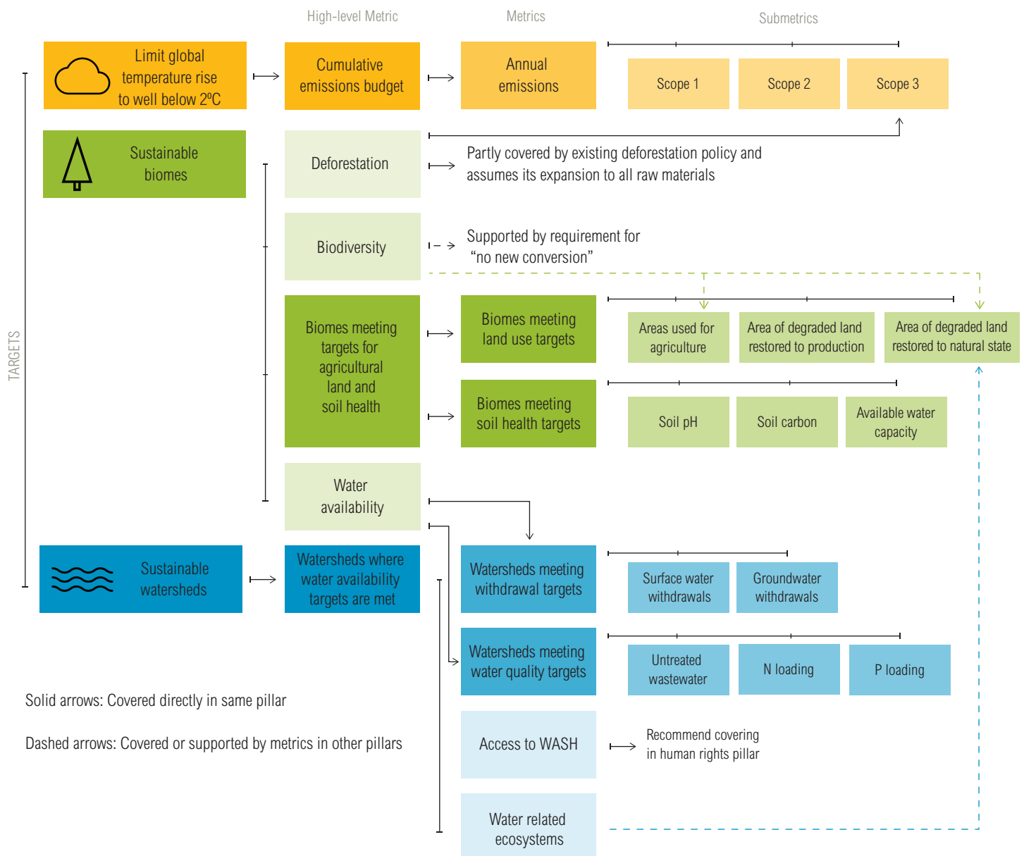
Figure A-1 | Ecosystem of Metrics: GHGs, Land, Water
