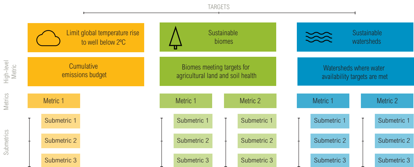
Figure 1. | Generic Example of a System of Supporting Metrics
