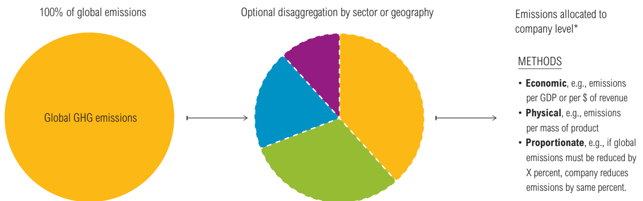
Figure 2 | Summary of Allocation Methods from the Science-Based Target Setting Manual
