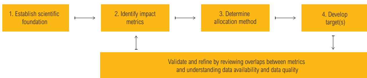
Figure ES-1 | Steps to Set Corporate Targets Anchored in Science for Multiple Environmental Impacts
