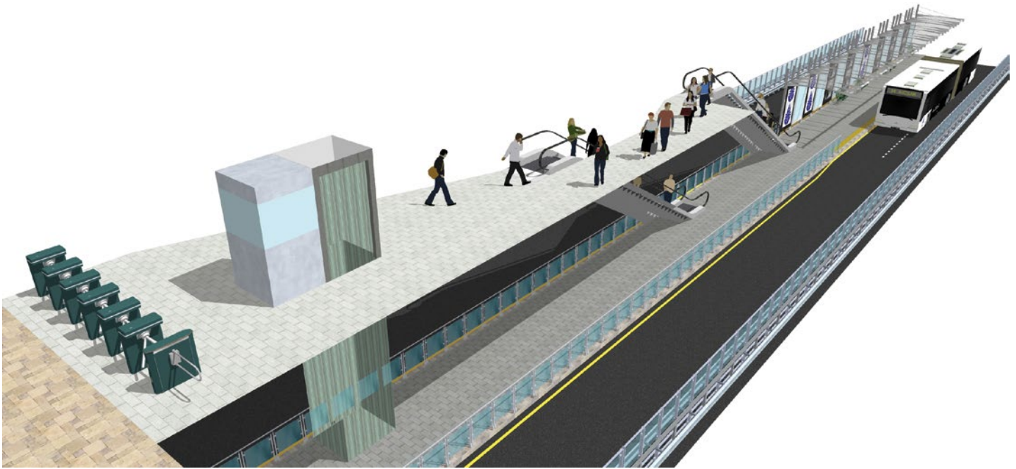
Figure 70 Design concept aimed at increasing passenger capacity and reducing overcrowding at a BRT station on the median of a freeway (note that this is a conceptual drawing of passenger access and does not show all the recommended guardrails)
