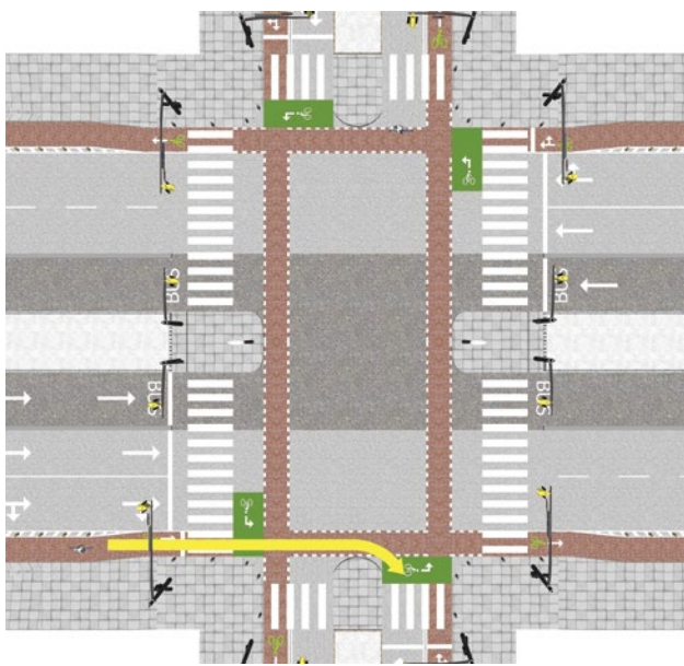
Figure 36 First stage of the left turn: Cyclists should continue straight along the BRT corridor on the green light, stop in the queue box to their right, and wait there for the light to change.
