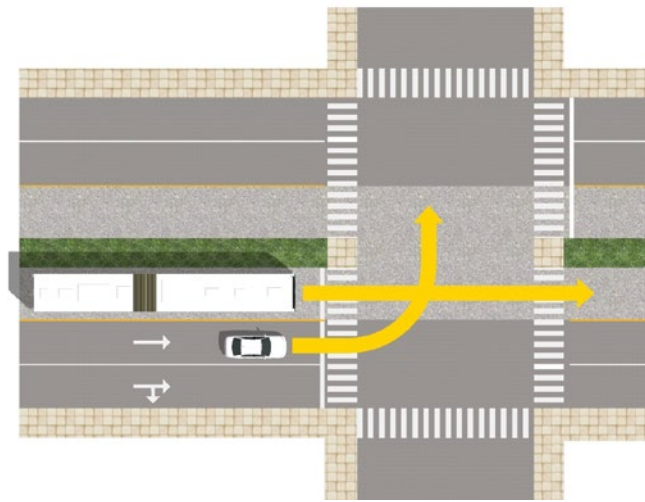
Figure 30 Crash diagram: The most common type of crash involving buses on center-lane BRT or busway corridors: Cars making illegal left turns in front of buses.
