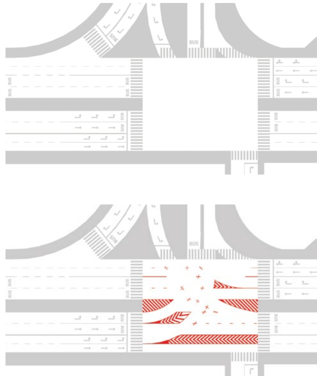
Figure 22 Example of an intersection with and without junction markings
