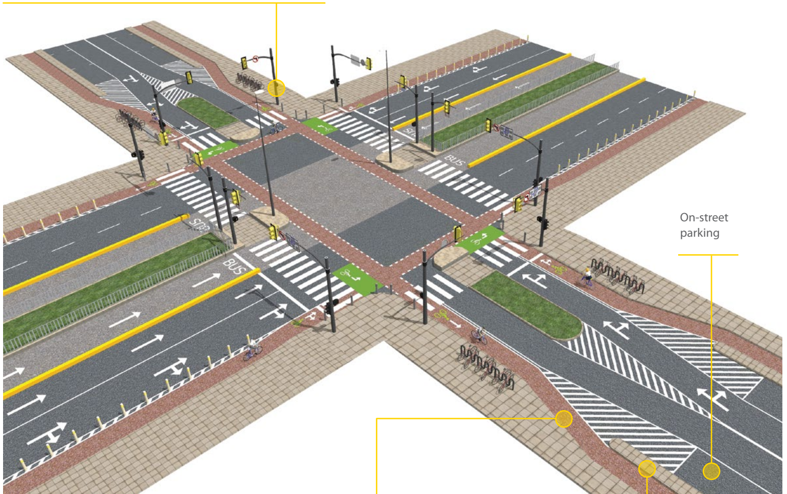
Figure 35 Minor four-way intersection, bike turns
