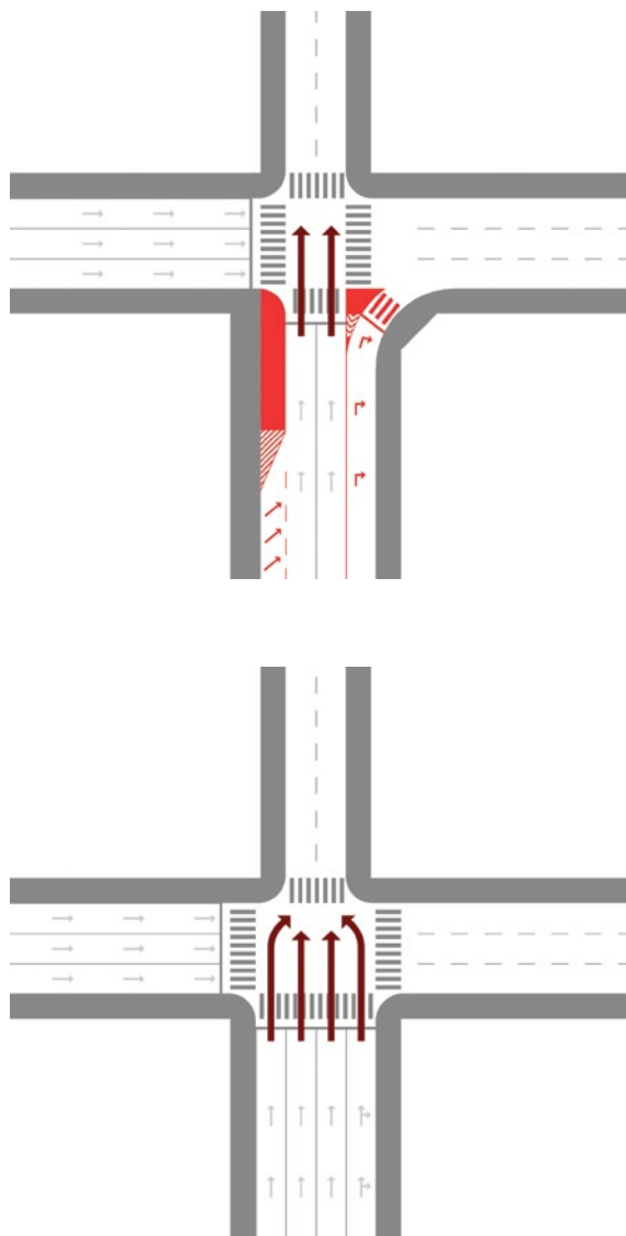
Figure 23 Example of how lane imbalance can be addressed by taking out lanes on one approach, or creating turn only lanes
