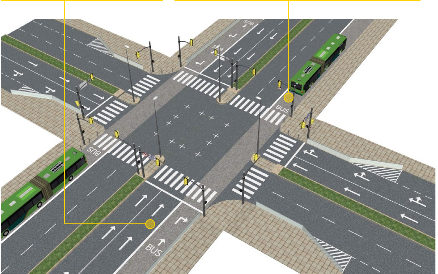
Figure 38 Curbside BRT intersection
