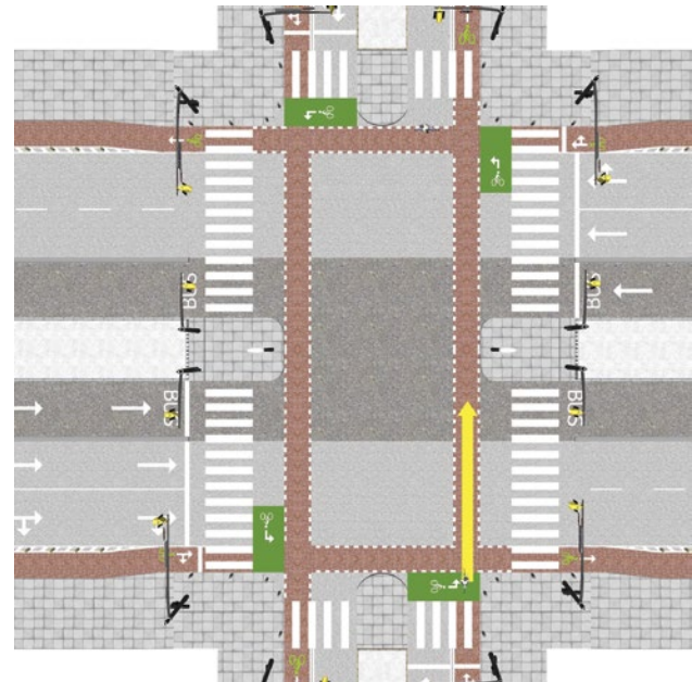
Figure 37 Second stage of the left turn: When the light turns green for the cross street, cyclists can cross the BRT corridor along with the rest of the traffic. Note the importance of the secondary traffic signal here. Cyclists will not be able to see the primary signal and will rely exclusively on the secondary one, situated on the far side of the intersection.
