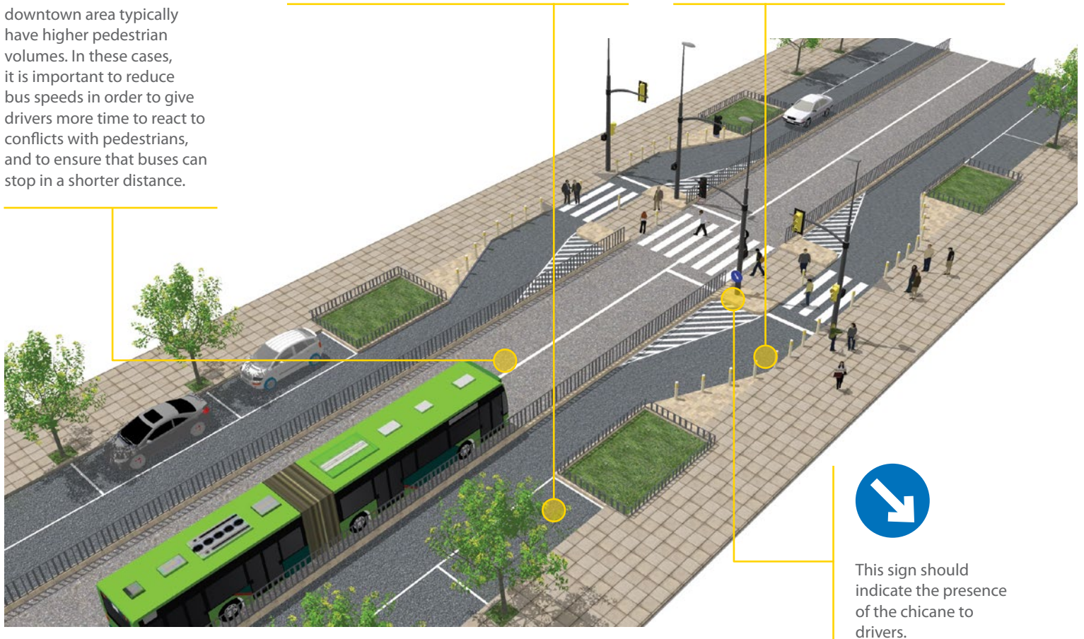
Figure 12 Midblock crossing on a narrow street
