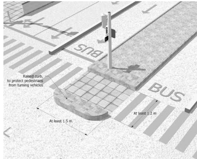
Figure 28 Detail of the pedestrian refuge island. The island should be at grade with the pavement and protected from traffic by a raised curb. It should provide sufficient space for the expected volume of pedestrians and at a minimum should accommodate a person with a stroller.
