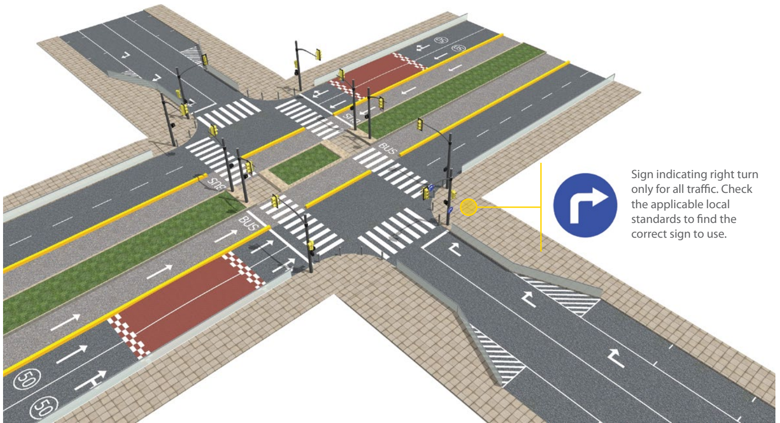
Figure 34 Blocked cross street
