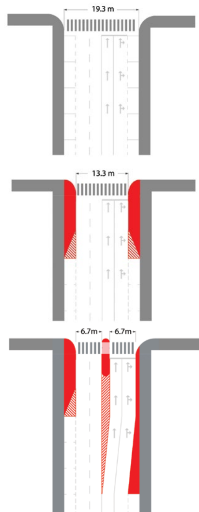
Figure 21 Daylighting and refuge islands
