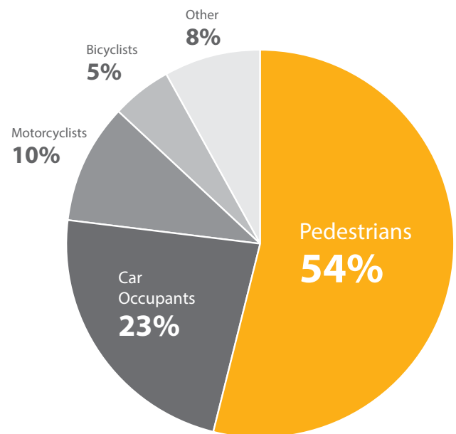
Figure 4 Fatalities on bus corridors by type of road user (includes data from Mexico City, Guadalajara, Delhi, Ahmedabad, Curitiba, Porto Alegre, and Belo Horizonte)
