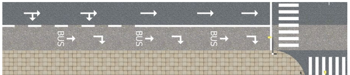
Figure 39 Plan view of one approach to the intersection along the bus corridor. Right-turning vehicles can merge into the curbside bus lane in advance of the intersection and then turn right from the bus lane. The space for merging into the bus lane should be at least 50 meters long.
