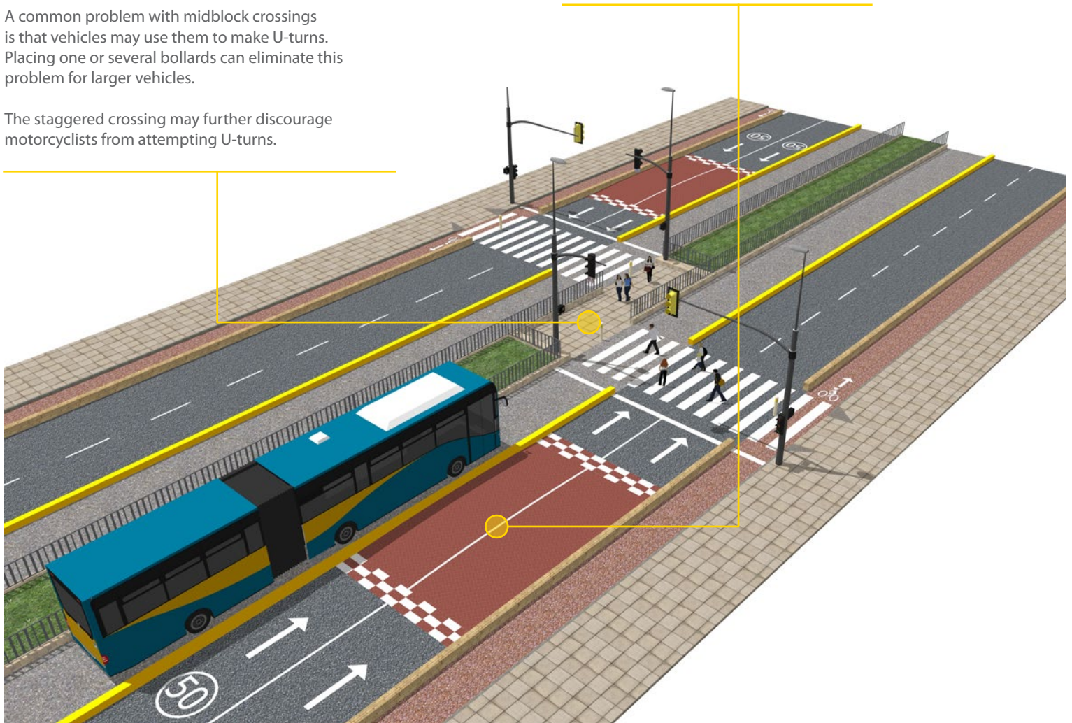
Figure 9 Midblock crossing on an urban arterial
