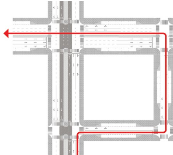
Figure 25 Loop option 2: Starting before the intersection with the left-turn prohibition
