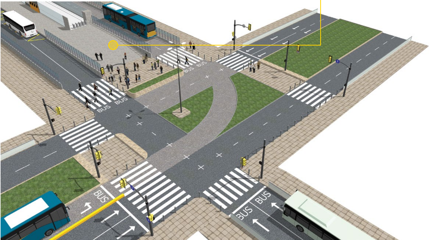
Figure 79 Access points to integrated terminals
