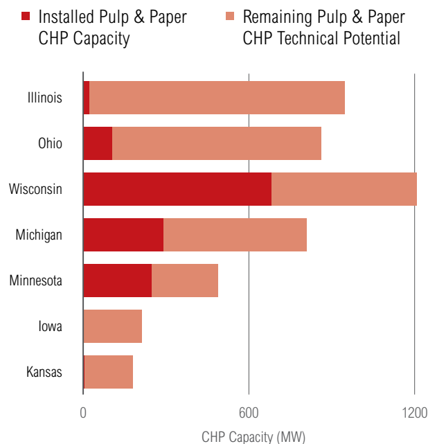
Figure 16 | Paper Sector Installed CHP Capacity and Estimated Remaining Technical Potential by State
