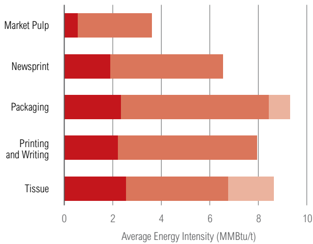
Figure 18 | Midwest Average Energy Intensity by Mill Type, 2010
