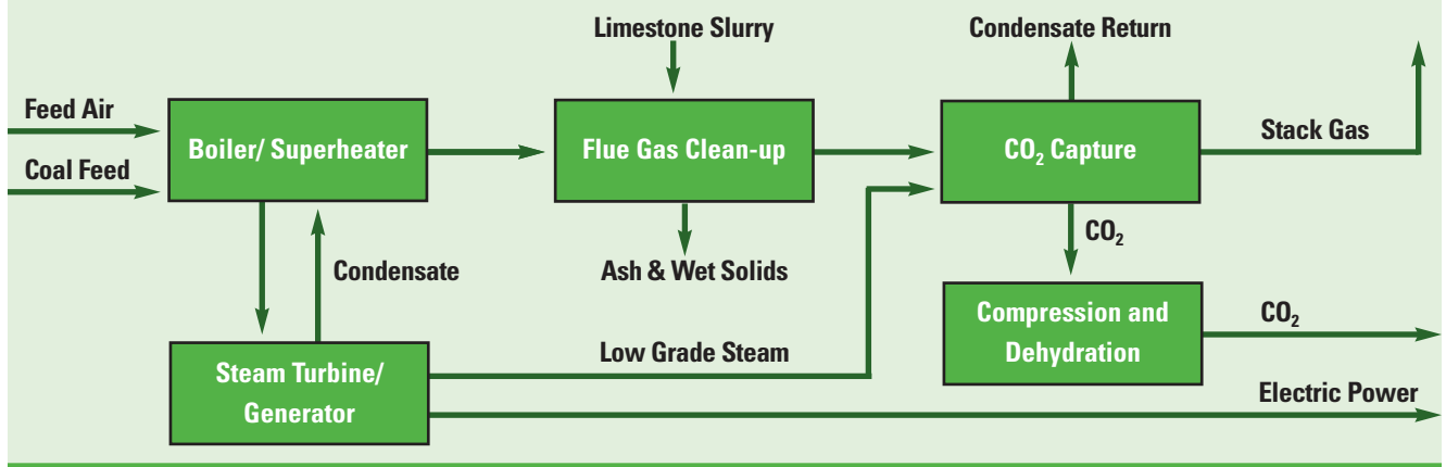
Figure 2: Post-Combustion Capture from a Pulverized Coal-Fired Power Plant
