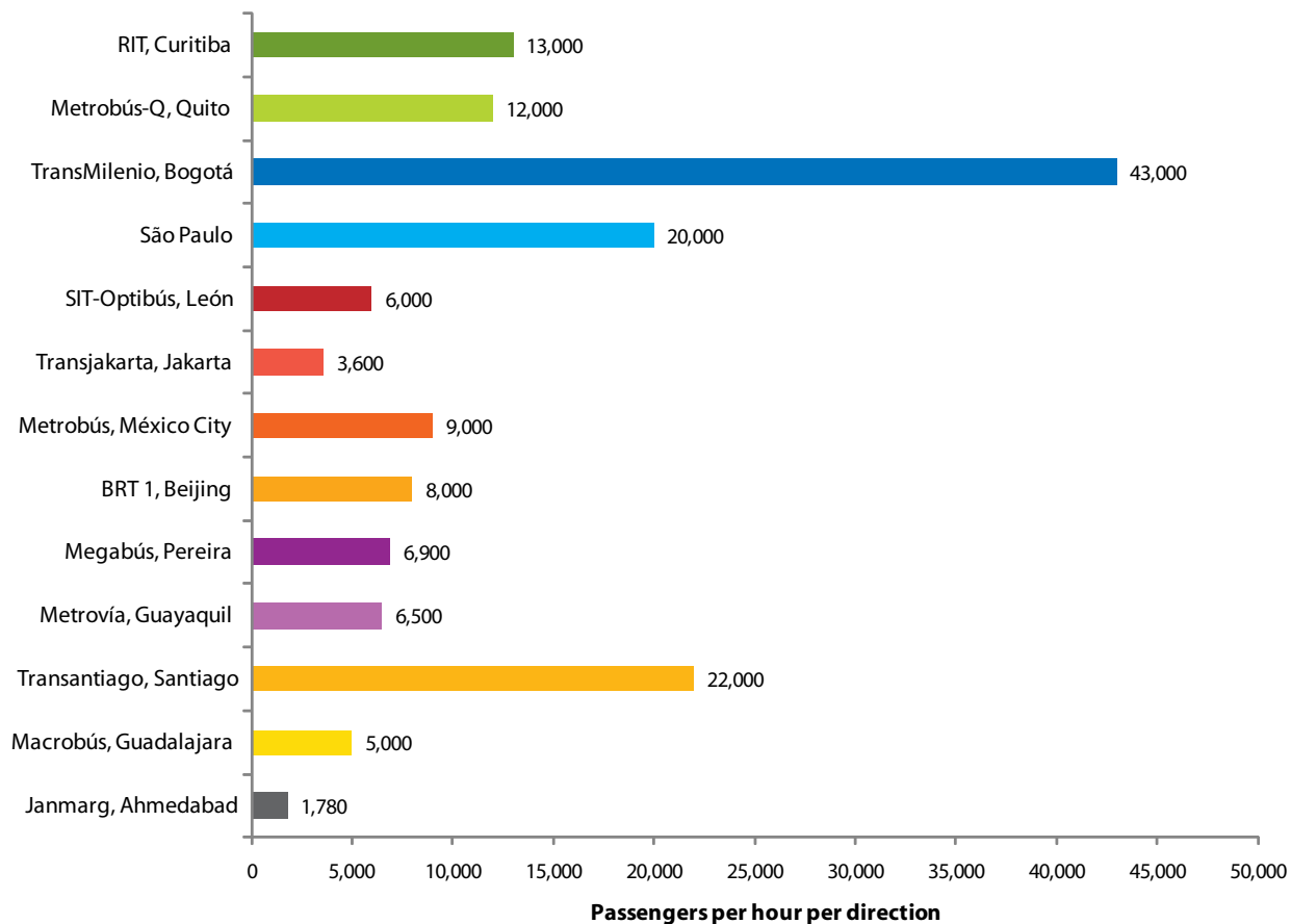
Figure 2 Peak Loads (2009)
